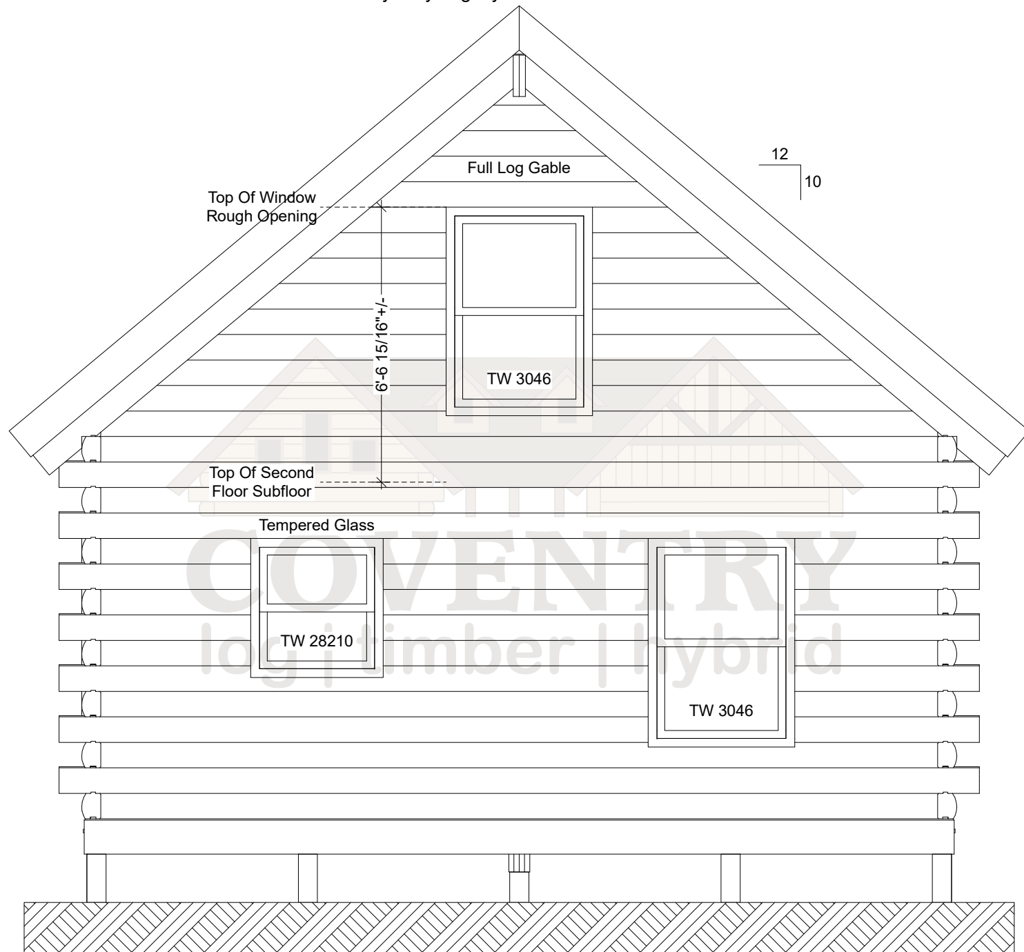
Northwood Left Elevation
