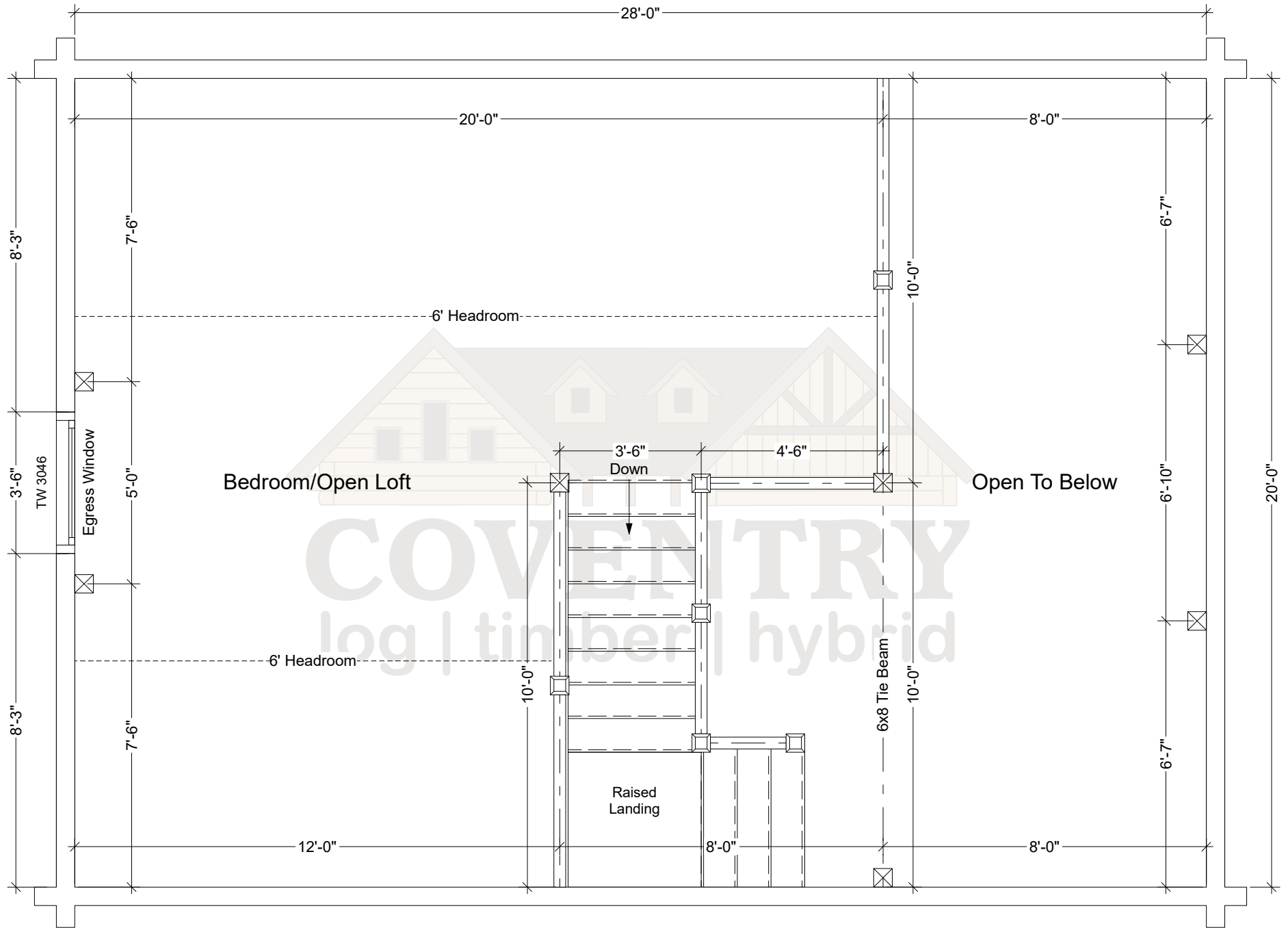
Northwood Second Floor Plan
