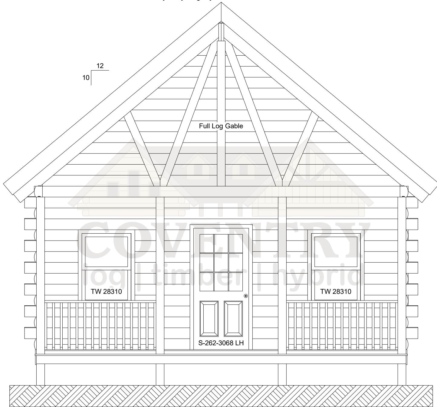
Northwood Right Elevation
