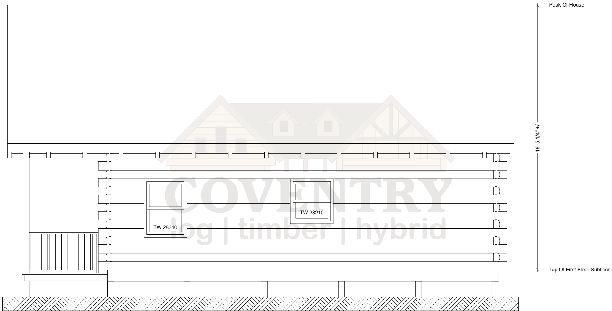
Northwood Rear Elevation
