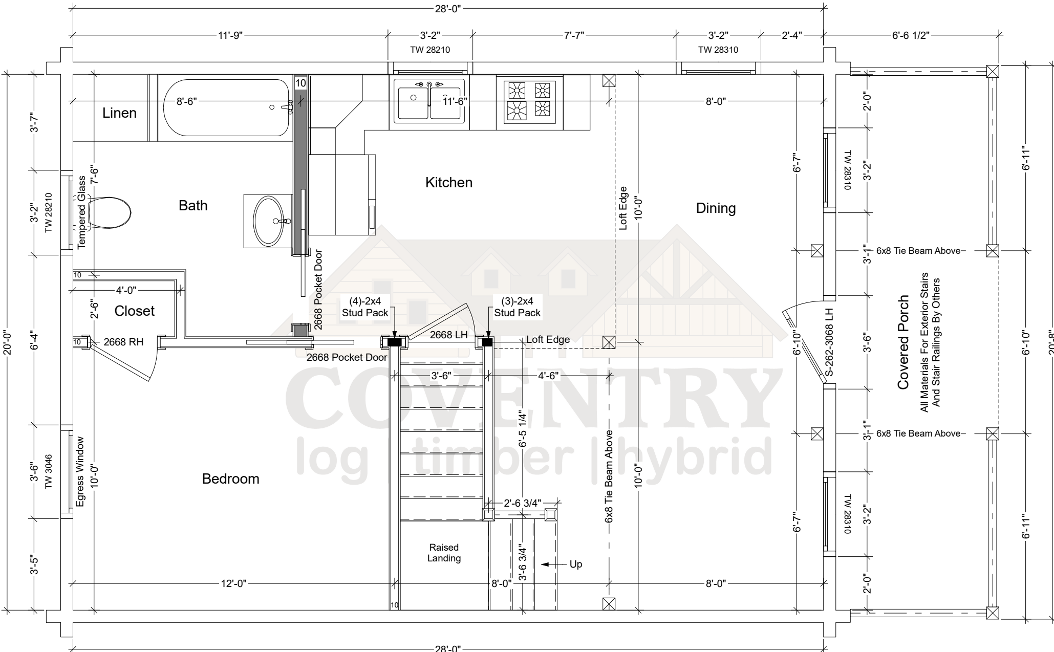
Northwood First Floor Plan
