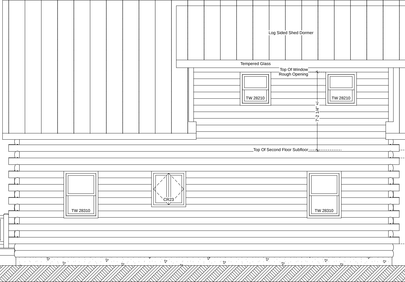
Skyline Right Elevation
