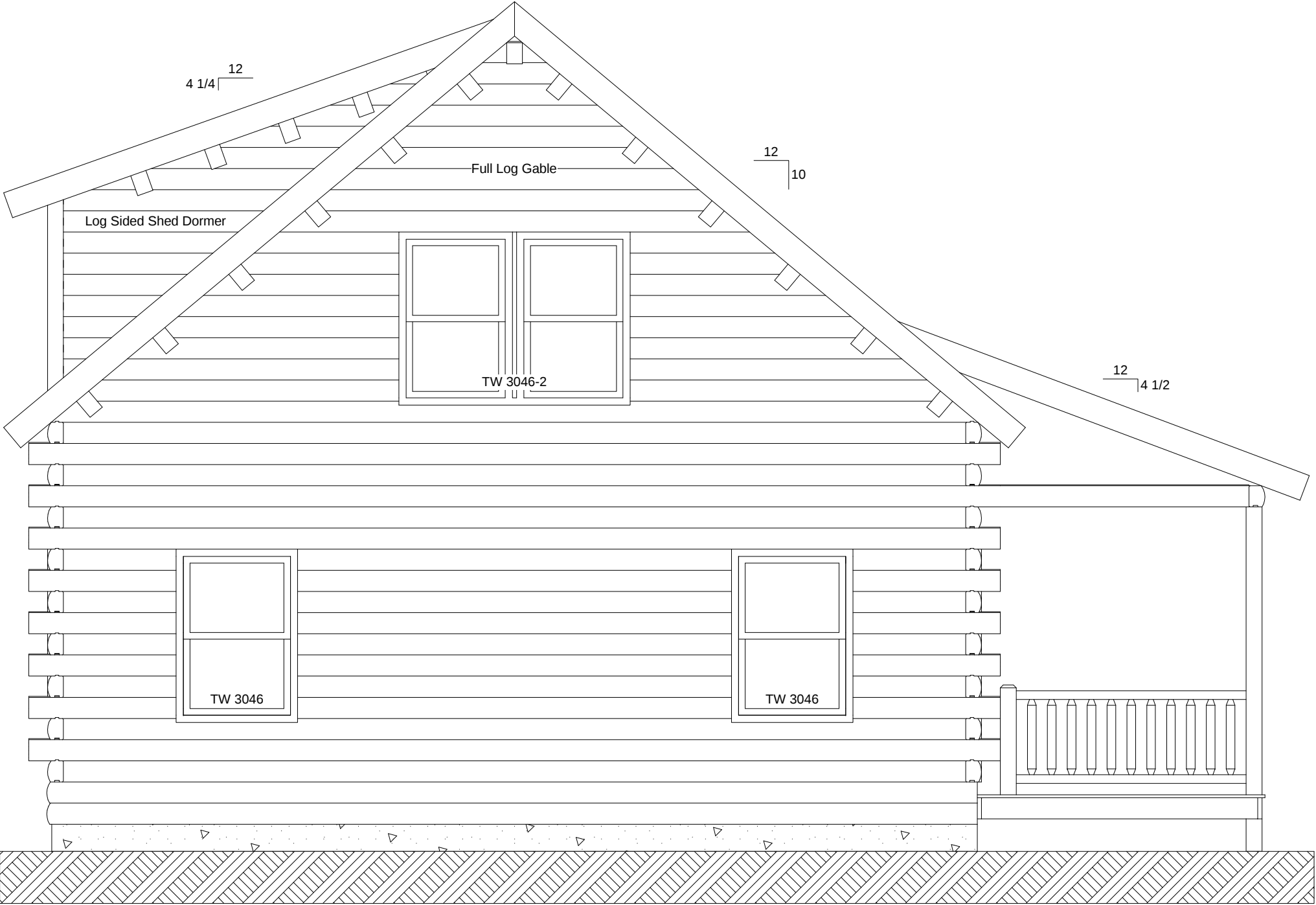
Skyline Rear Elevation
